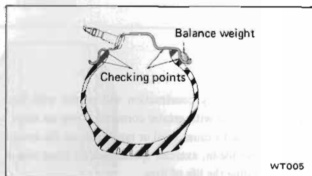
Fig. WT-4 Wheel rim run-out checking points
