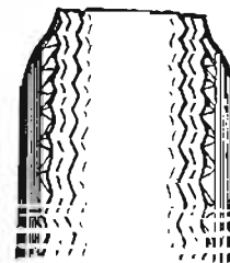
Overinflation wear
