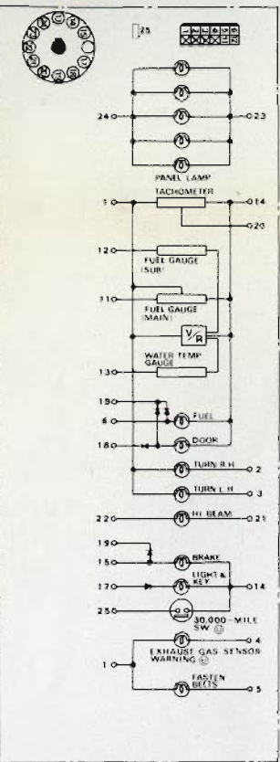
COMBINATION METER
