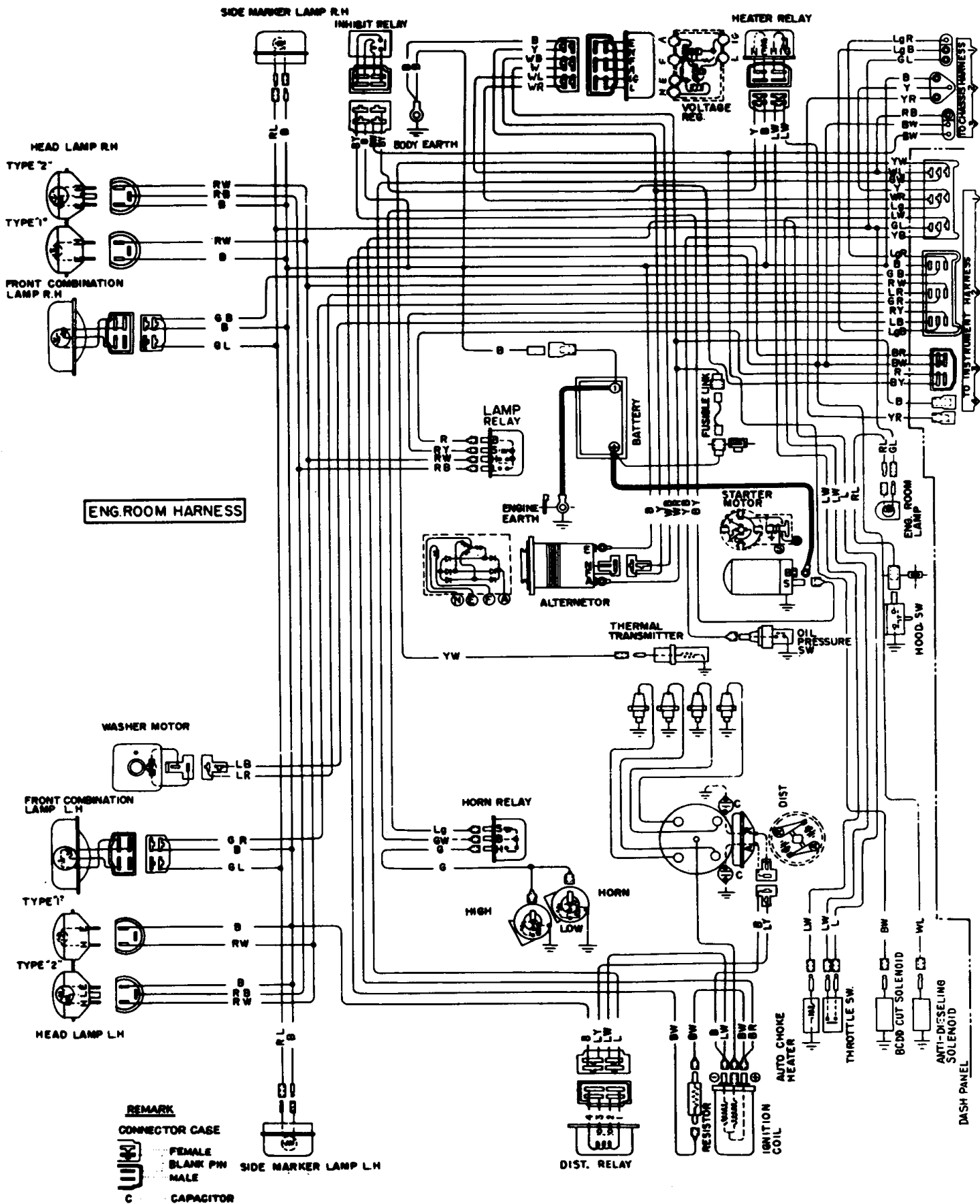
Fig. 10.35. Wiring diagram - 1973 USA - automatic transmission
