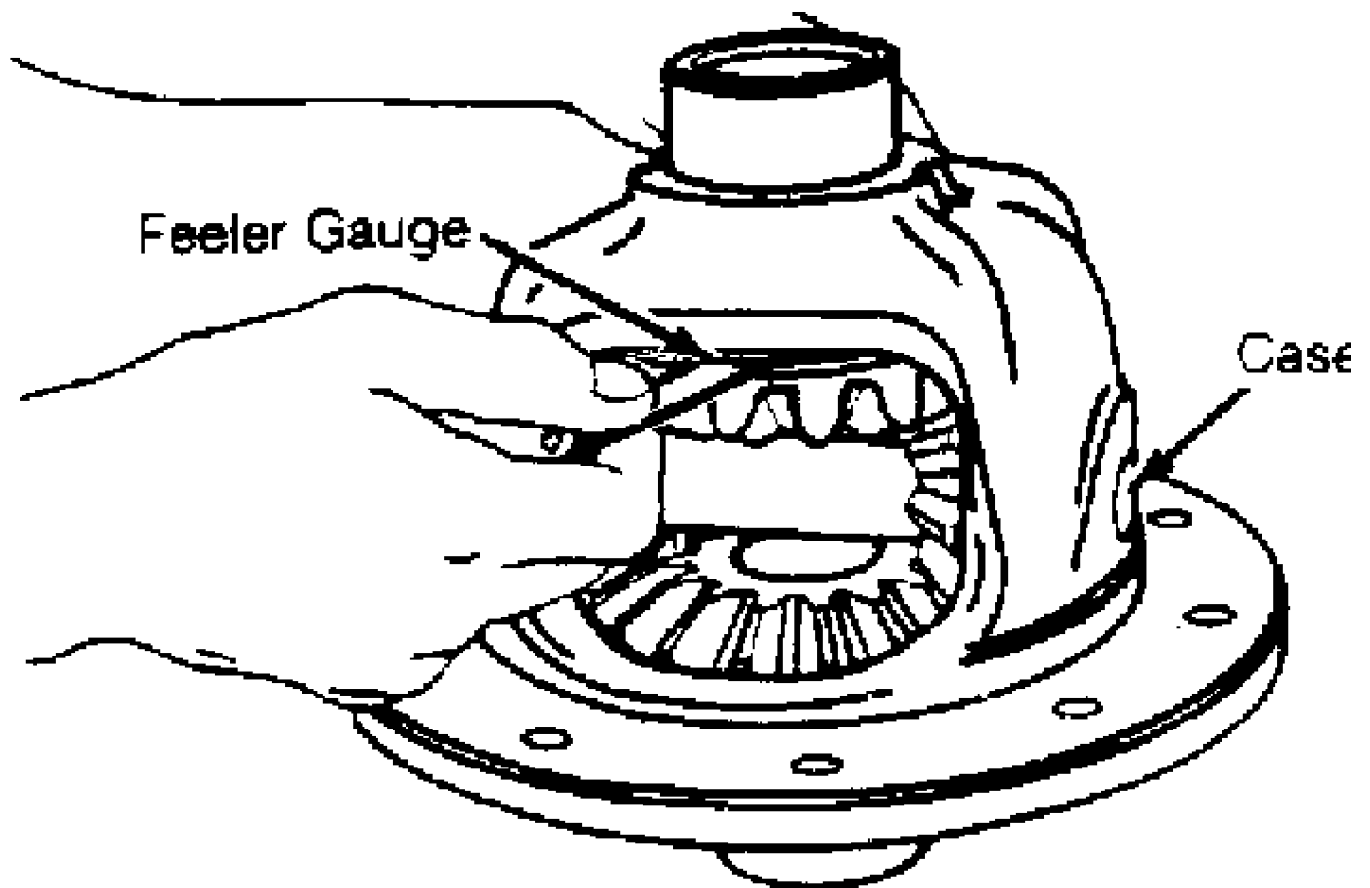
Fig. 3: Measuring Side Gear-to-Thrust Washer Clearance Courtesy of Nissan Motor Co., U.S.A.
