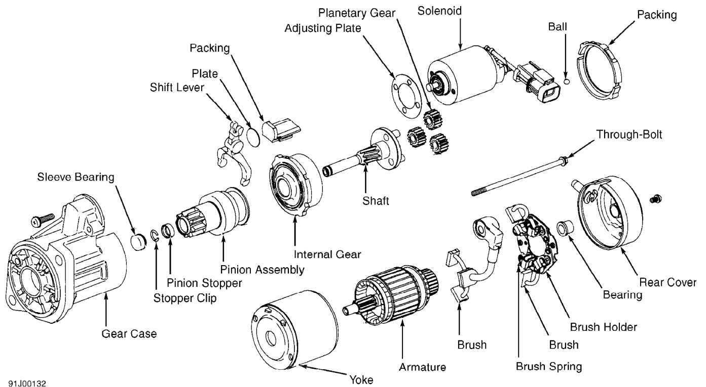
Fig. 2: Exploded View of Starter M1T60281 (M1T72781 for 240SX is Similar)
