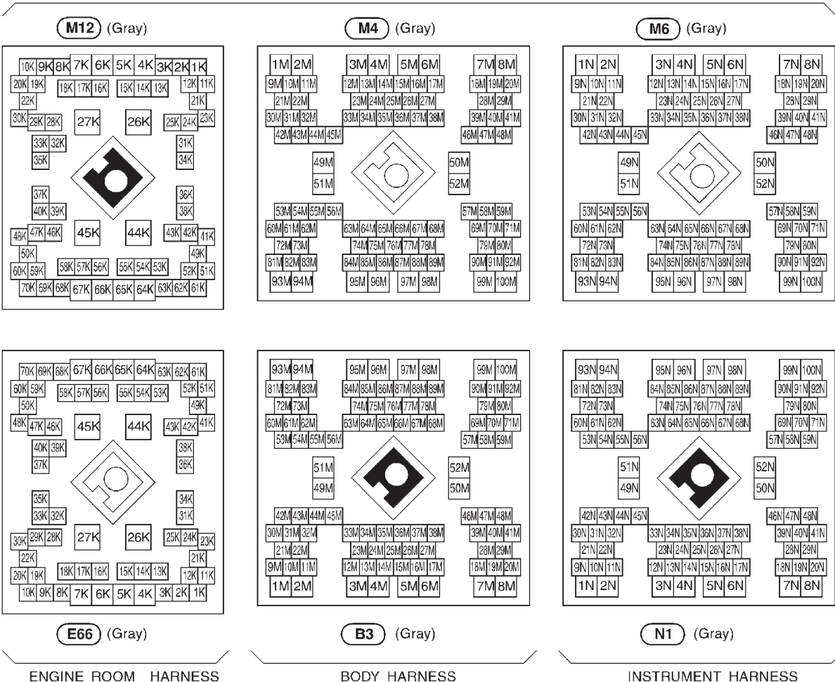
ENGINE ROOM HARNESS
